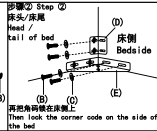
图2: 角码安装示意图 Figure 2: installation diagram of corner code
