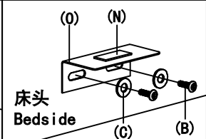
图3: 新5号角码安装示意图 Figure 3: installation diagram of new No. 5 corner code
