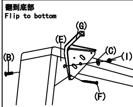
图1: 床脚安装示意图 Figure 1: installation diagram of bed foot
